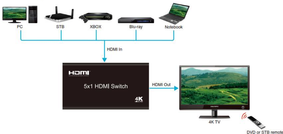
Connection Diagram
